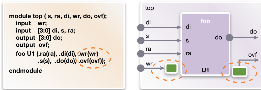
Figure 4: Example of an RTL instantiation that has more pins than the block it references
