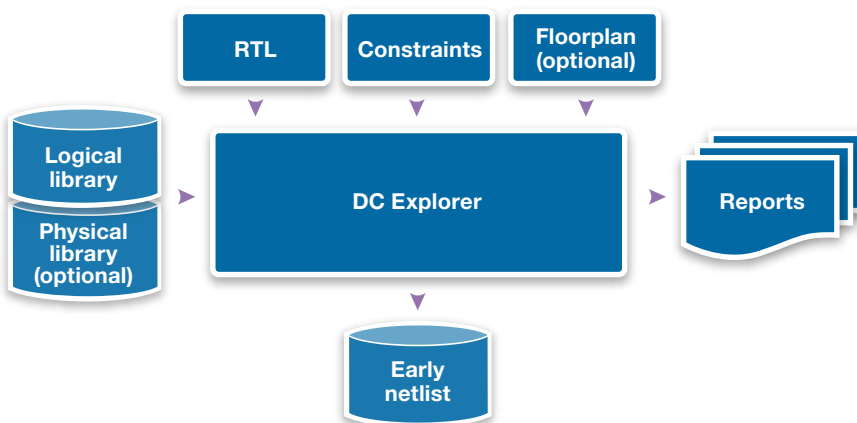
Figure 12: DC Explorer inputs and outputs
