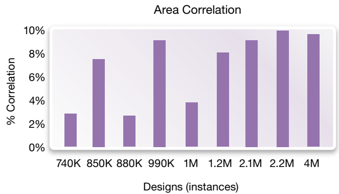
Figure 10: DC Explorer delivers 10% area correlation to DC Ultra (Topographical)
